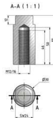
Collar nut M12/M16 Art. No. 2031-400
