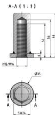
Collar nut M12/M16 Art. No. 2032-A4
