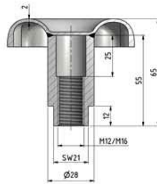
Stainless steel handle Art. No. 2022/3022
