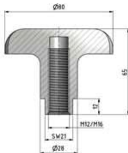
Stainless steel handle Art. No. 2022V / 3022V
