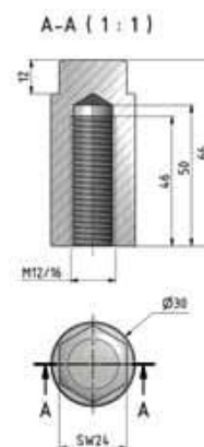
Collar nut M12/M16 Art. No. 2032-400
