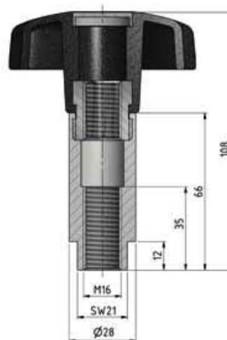
Plastic handle Art. No. 2016L
