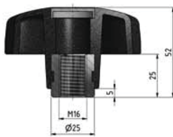
Plastic handle Art. No. 2016
