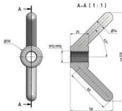
V-toggle M12/M16 Art. No. 2023 / 2023-A4
