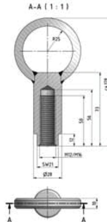
Ring nut M12/M16 Art. No. 2023RS / 2023RS-A4
