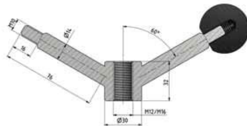
V-toggle M12/M16 Art. No. 2023K / 2023K-A4
