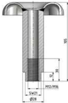
Stainless steel handle Art. No. 2022L / 3022L
