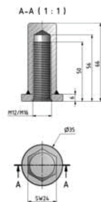
Collar nut M12/M16 Art. No. 2032
