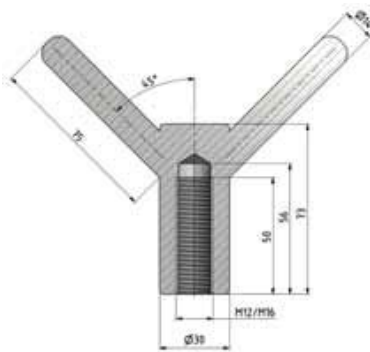
V-toggle M12/M16 Art. No. 2023S / 2023S-A4
