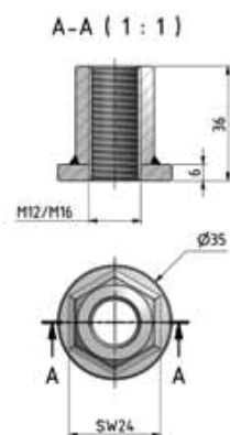
Collar nut M12/M16 Art. No. 2031
