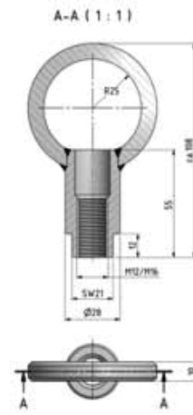
Ring nut M12/M16 Art. No. 2023R / 2023R-A4
