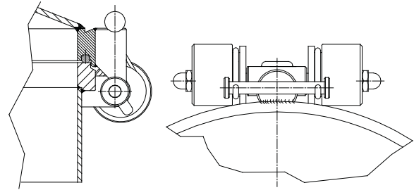
Spring assist with torsion springs (single version)
