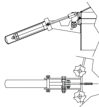
Spring assist with Gas-Spring (single version)
