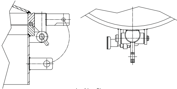
Locking Pin
