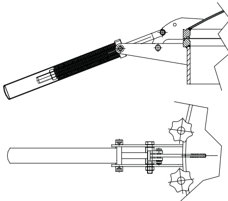
Spring assist with Disc-Springs (single version)
