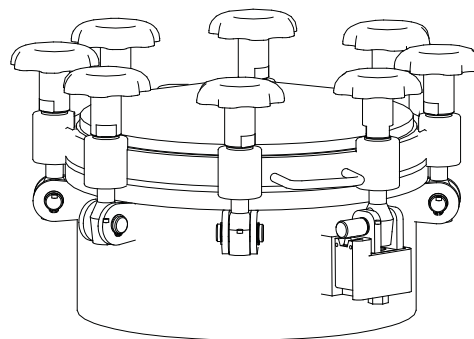
Screw with safety device Article No. 2027SK
